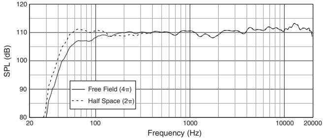
Frequency Response
